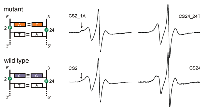
FIGURE 6: EPR spectra of R5a at positions 2 and 24 in the mutant (top) and wild type (bottom) CS duplexes. Arrows indicate immobilized spectral components. CS2_1A, CS24 and CS24_24T spectra were corrected for the presence of the residual free nitroxide ( < 3\% ).
