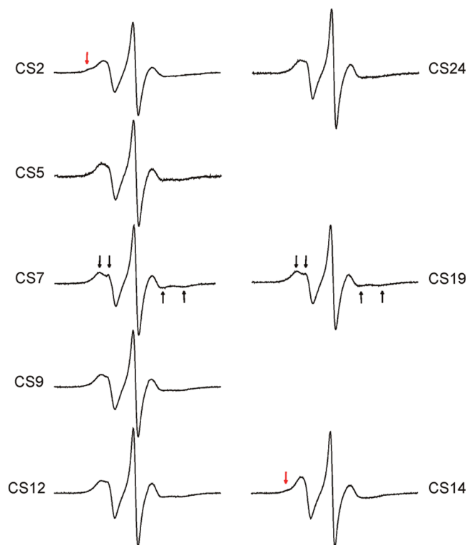
FIGURE 5: EPR spectra of R5a labeled CS DNA duplexes. Black arrows indicate the resolved hyperfine extrema at CS7 and CS19. Red arrows indicate the presence of a second spectral component at CS2 and CS14. Spectra of CS9, 12, 14, 19, and 24 were corrected for the residual free nitroxide ( < 3\% ).
