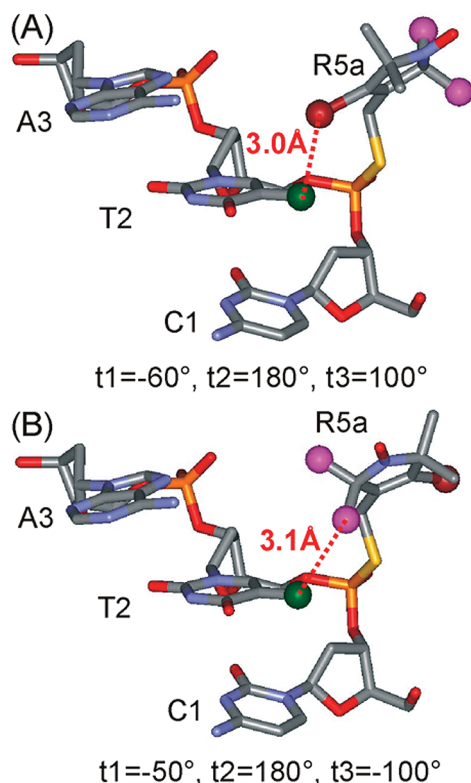
FIGURE 8: Proposed R5a/DNA interactions at the 5' terminal site CS2. The models were generated using WebLab ViewerPro 3.7 (Molecular Simulations, Inc.), with R5a attached to the R_p phosphorothioate of the target site in the NMR structure of the CS duplex. The 4-Br atom of R5a is shown as a dark red ball, the C2 methyls of R5a are shown as purple balls, and the C5-methyl of T2 is shown as a green ball. In the modeling, the torsion angle t_1 was varied, while t_2 and t_3 were set based on MD simulation data, which show t_2 \equiv 180^\circ ; and t_3 = +100^\circ or -100^\circ . (A) R5a modeled with t_1 = -60^\circ , t_2 = 180^\circ , and t_3 = +100^\circ . This particular t_1 value gives the closest distance between the 4-Br atom of R5a and the C5-methyl of T2 without any steric collision between R5a and DNA. (B) R5a modeled with t_1 = -50^\circ , t_2 = 180^\circ , and t_3 = -100^\circ . This configuration gives the closest distance between one of the 2-methyl groups of R5a and the C5-methyl of T2 without any steric collision.
